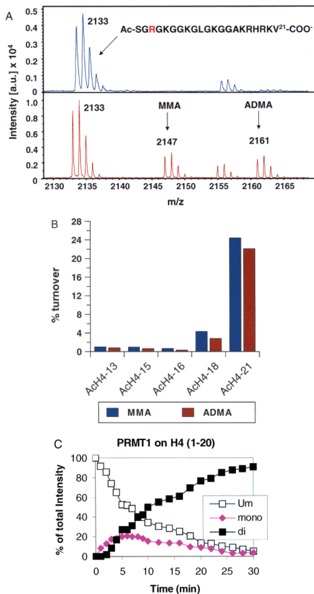
FIGURE 3: rPRMT1 catalyzes H4 Arg3 methylation in a partially processive fashion. A. Methylation of the AcH4-21 peptide monitored by MALDI-MS. B. Comparison of the relative levels of monomethylated and dimethylated peptides produced as a function of peptide length. The concentrations of SAM and rPRMT1 were fixed at 250 \mu M and 500 nM, respectively. The concentrations of the peptide substrates were fixed at \sim 2.5K_m (AcH4-13 = 275 \mu M; AcH4-15 = 310 \mu M; AcH4-16 = 370 \mu M; AcH4-18 = 500 \mu M; AcH4-21 = 9 \mu M). C. Time course of rPRMT1 catalyzed methylation. Methods analogous to those described in (66) were used for these studies. The relative amount of each peptide species over the full time course of the reaction was expressed as a percentage of the sum of intensity of all related peaks. The methylation reaction contained 20 mM Tris pH 8.0, 200 mM NaCl, 1 mM DTT, 0.4 mM SAM, 20 \mu M of peptide, and 50 \mu g/mL of PRMT1 and was carried out at 37 ^{\circ} C.
