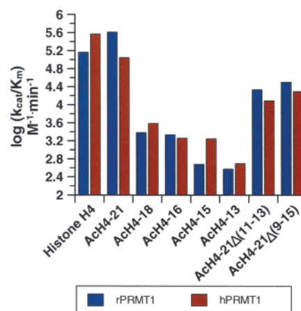
FIGURE 2: Substrate specificity of human PRMT1 versus rat PRMT1. The k_{cat}/K_m values determined for histone H4 and histone H4 based peptides of varying length are depicted graphically.
